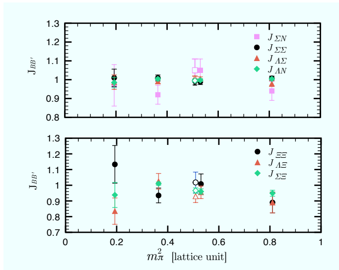
FIG. 6: J_{BB'} as defined in Eq. (13) as a function of m_\pi^2 .
