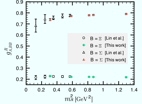
FIG. 4: Comparison of our results for g_{A,\Sigma\Sigma}^R and g_{A,\Xi\Xi}^R with those in Ref. [10]
