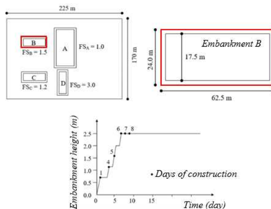
Figure 1. The location plan of test embankments, geometrical dimensions and construction process of embankment B
