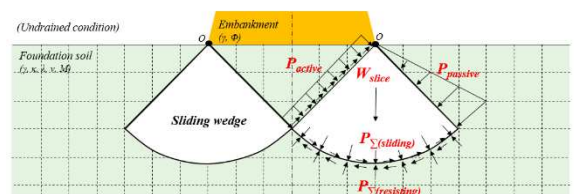
Figure 6. A representative sliding wedge
