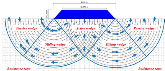
Figure 3. The general failure mechanism drawn for the proposed method
