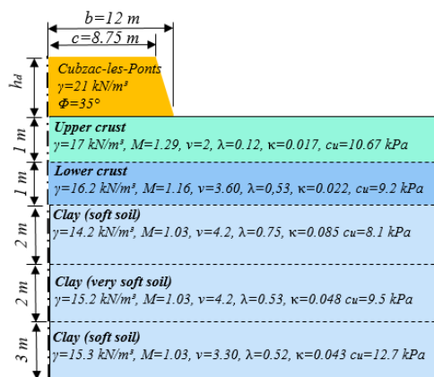
Figure 2. Geotechnical and geometrical properties of the embankment B.
