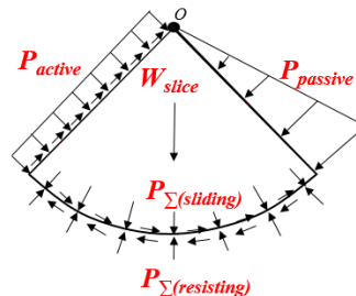
Figure 7. The stresses and forces acting on the first local failure slice
