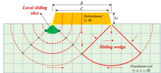
Figure 5. Development of local sliding mechanisms
