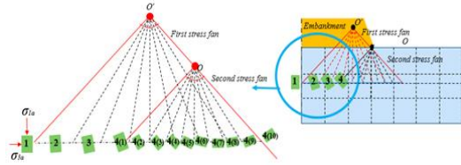
Figure 4. Dual stress rotation effect considered by two slip fans.
