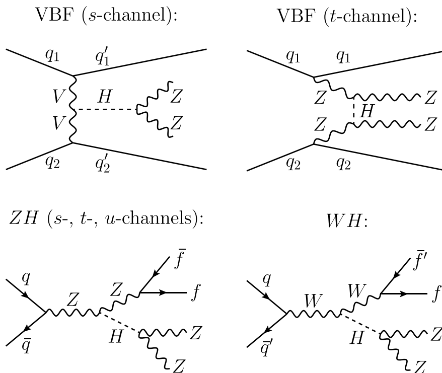
Extended Data Fig. 1 | Feynman diagrams for the H boson-mediated EW ZZ production contributions. Here, f refers to any \ell , \nu , or q . The tree-level diagrams featuring VBF production are grouped together in the upper row, and those featuring VH production are grouped in the lower row. The interaction displayed in each diagram is meant to progress from left to right. Each straight, curvy, or curly line refers to the different set of particles denoted. Straight, solid lines with no arrows indicate the line could refer to either a particle or an antiparticle, whereas those with forward (backward) arrows refer to a particle (an antiparticle).
