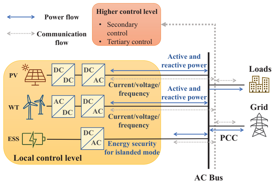
Figure 3. Basic hierarchical control structures adapted from [43].
