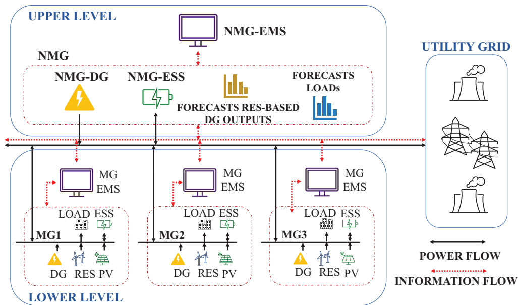
Figure 8. The basic NMG structure.
