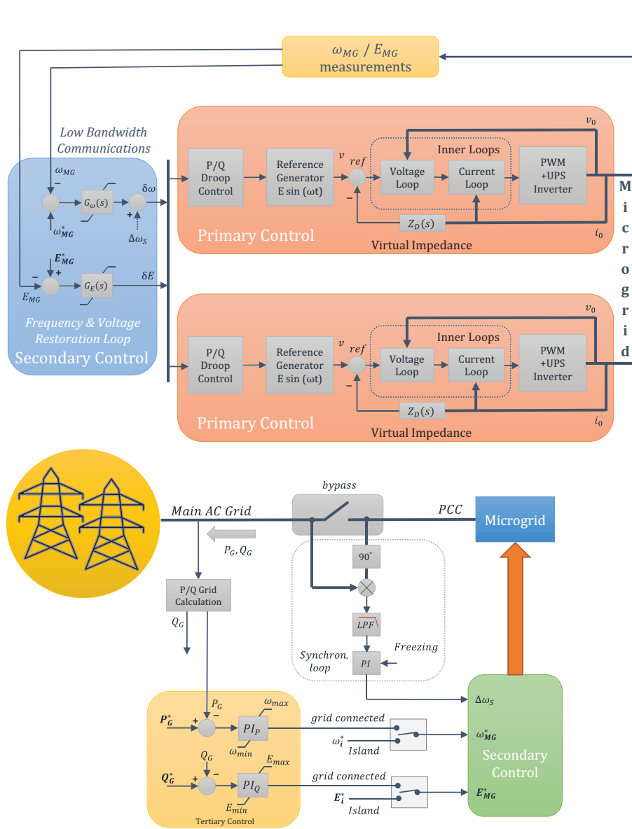
Figure 1. Block diagrams of the hierarchical control of an ac MG adapted from [48].
