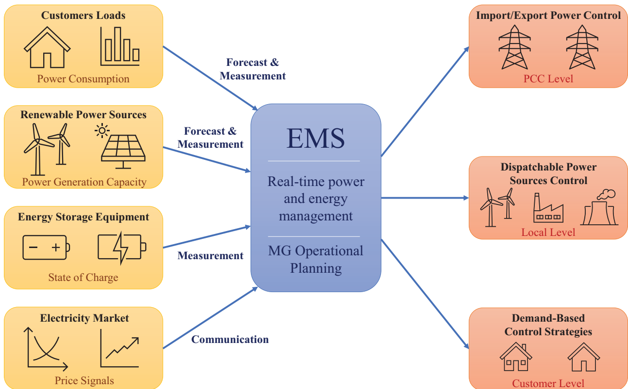
Figure 7. Energy management systems adopted from [149].
